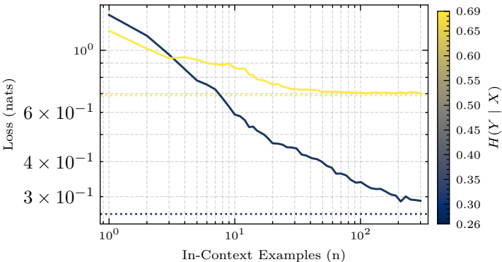
In-Context Learning Loss for Qwen-2.5 (1.5B)
